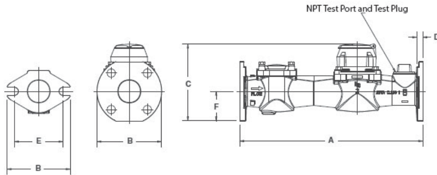
Figure 2: Physical dimensions
